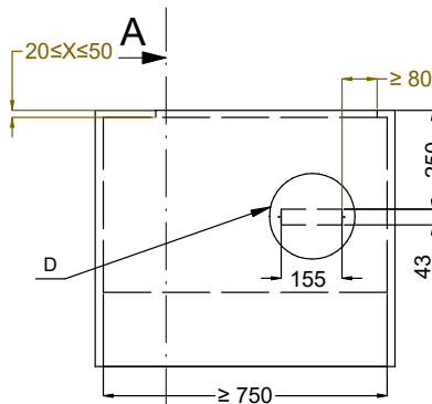
Front view Scala: 1:10
