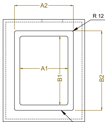
Top view Scala: 1:10
